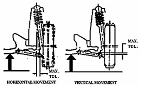
MACPHERSON STRUT
