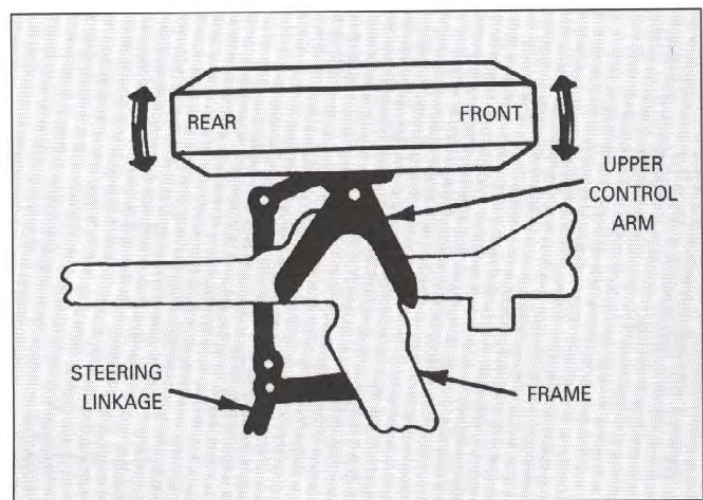
Steering Linkage Play—Top View
