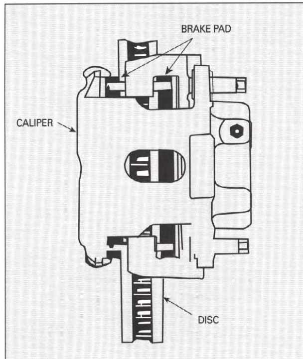
Typical Disc Brake
