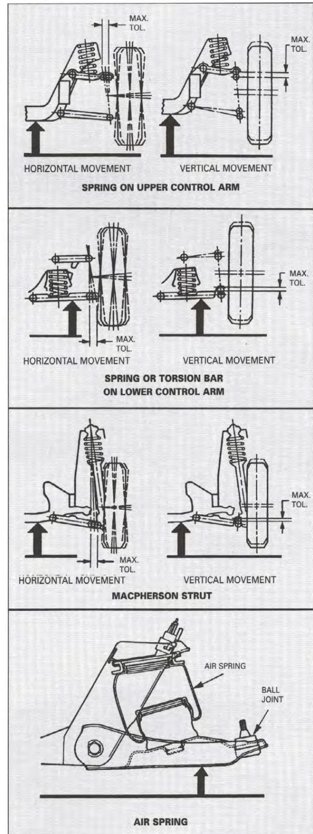
Raising Positions for Suspension Systems
